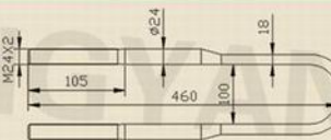
规格/SIZE M24 X 2 X 100 X 460
