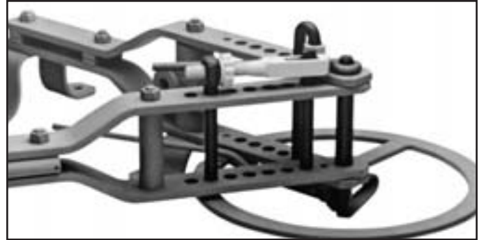
16B Eye-Bolt Bending Dog, toe to front, bending small-diameter Eye Bolt around 20B Center Pin on top of bender
