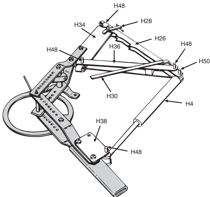
49126 H4 Hydraulic Cylinder Assembly and 49350 Hydraulic Conversion Kit
