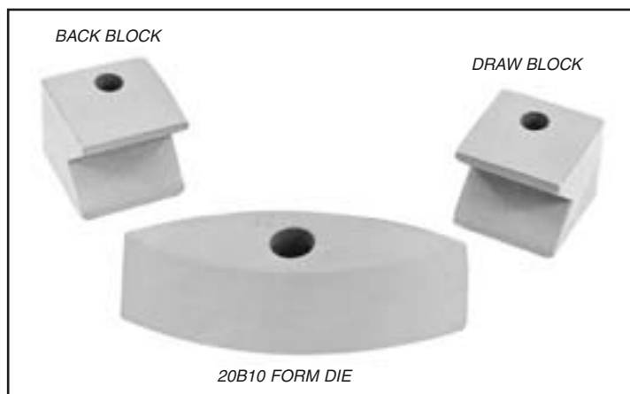
20B10 Form Die with 42990 Back Block/Draw Block Set bending Angle Iron with the "Heel Out"
