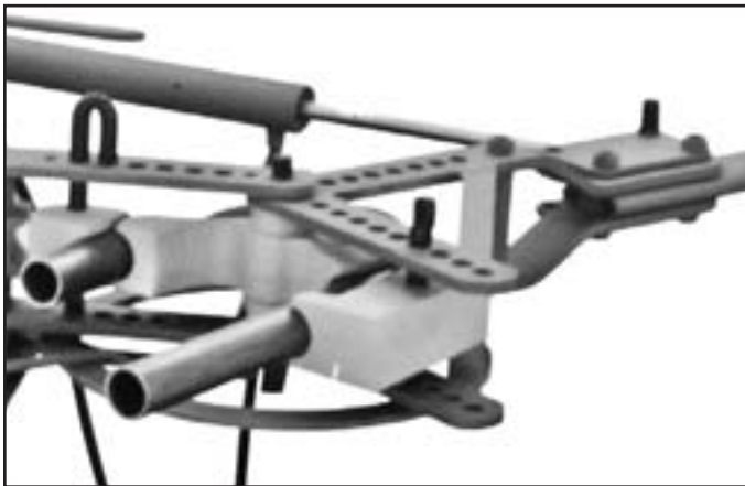
"L-Type" Swinging Frame bends 2" Pipe a full 180° using a 180° wrap-around-type die
