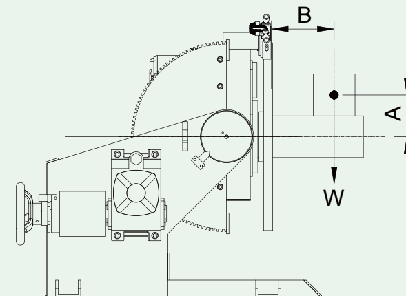
WPT-5FB Positioner Eccentric Load
