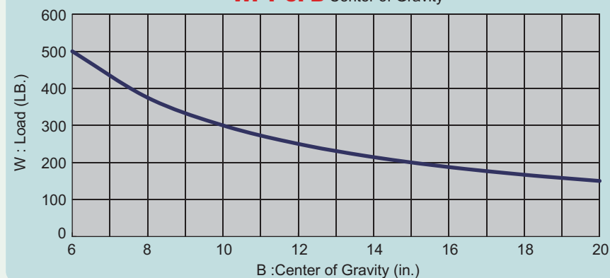
WPT-5FB Center of Gravity
