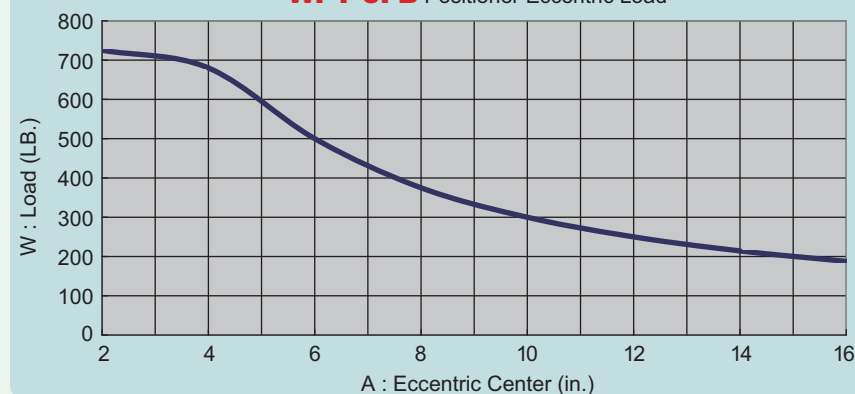
WPT-5FB Positioner Eccentric Load
