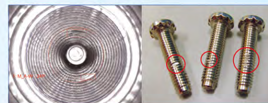
螺牙360° 檢測之照片 360° Degree Thread Damage Inspection (Customized)
