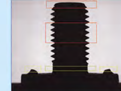
焊點高度/桿徑/螺牙 welding points/width/pitch
