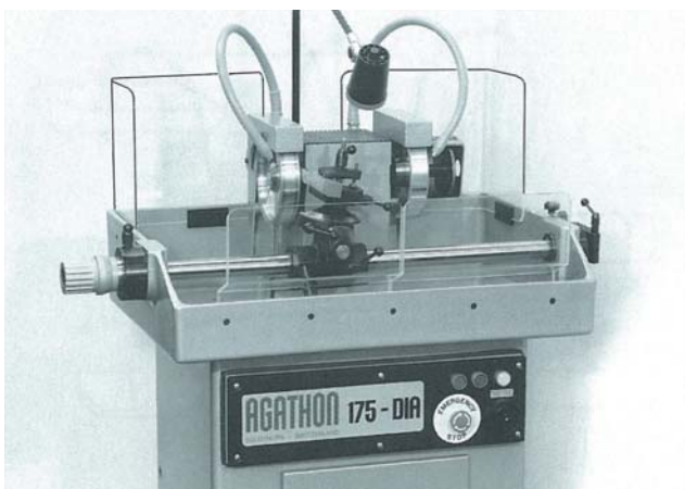
Effective 4-piece plexiglass splash guards, items 2.00.96.60, ...80
