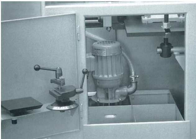
The high capacity coolant pump is mounted directly on the pull-out coolant tank
