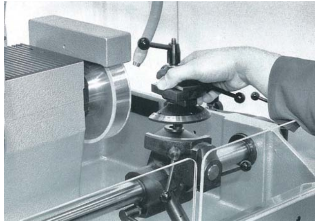
Rapid changeover of accessories. Tool holder 15, item 3.00.49.40, placed in basic adapter
