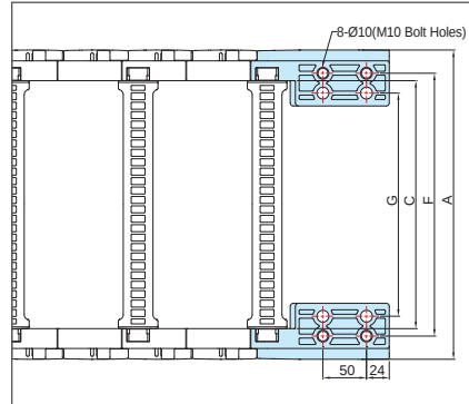
Fixing point
