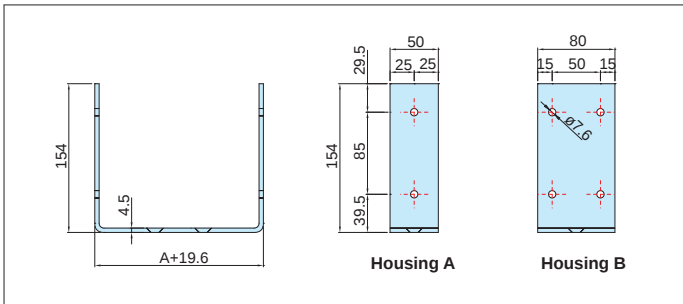
Housing (U-shape)
