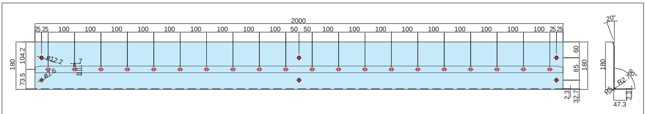
Side Panel
