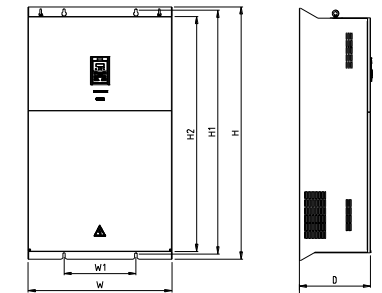
c) GK800-4T90~GK800-4T185
