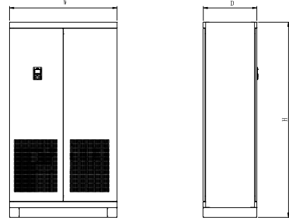
f) GK600-4T560G/630L~GK600-4T630G/710L
