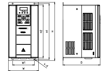
b) GK600-4T2.2G/3.7LB~GK600-4T15G/18.5LB
