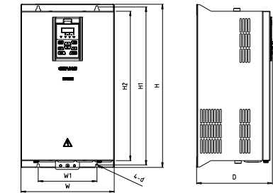
b) GK800-4T18.5~GK800-4T75
