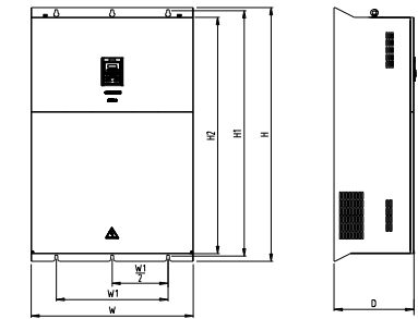
d) GK800-4T200~GK800-4T400
