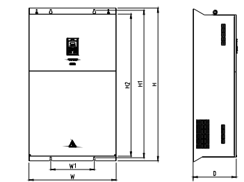
d) GK600-4T90G/110L~GK600-4T185G/200L
