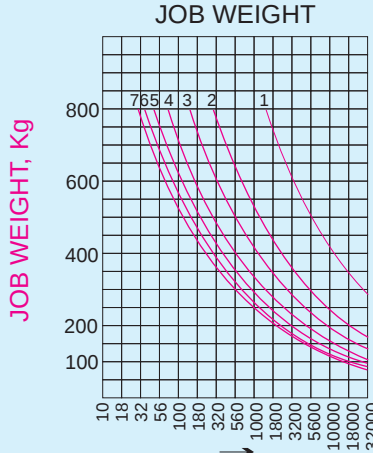
SERVICE LIFE OF MT4 BEARING ARRANGEMENT IN HOURS
