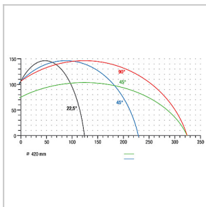
Mitre saw MGS 105 Cutting diagram MGS 105
