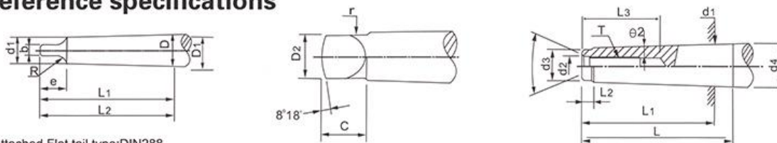
A Attached Flat tail type: DIN288
