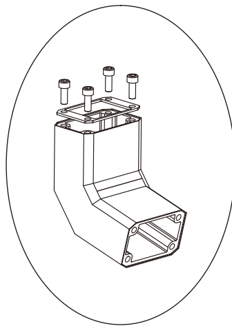
硬連接 Hard Joint
