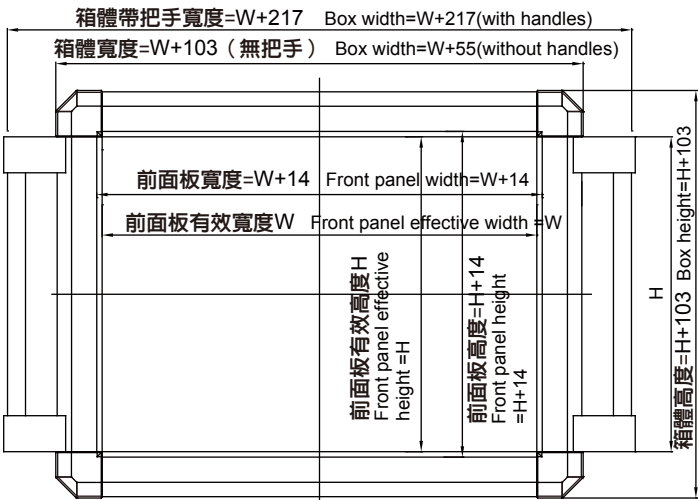
DST210 箱體尺寸(兩側把手) DST210 box size (handles on both sides)
