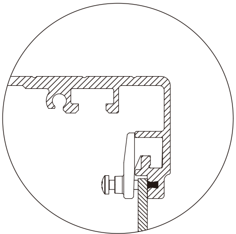
箱體上下側面板安裝 Installation of the front panel on upper and lower side
