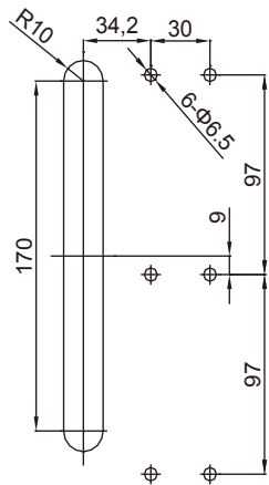
箱體安裝孔尺寸 Mounting hole size of the box
