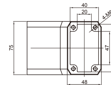
硬連接內孔尺寸 Bore size of the hard joint
