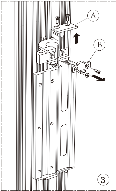
2. 卸下A和B兩個小蓋板。 Remove the two small cover plates A and B.
