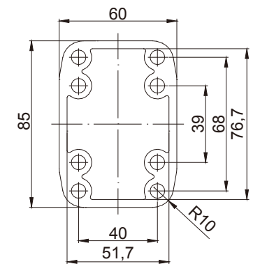
6085鋁管規格表(配6085懸臂)： Size table of 6085 aluminum tubes ( for 6085 support arms)
