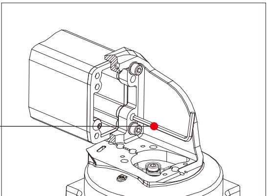
調節連接管水平度 Adjusting levelness of the connecting tube
