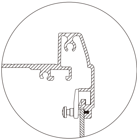
箱體左右側面板安裝 Installation of the front panel on left and right side
