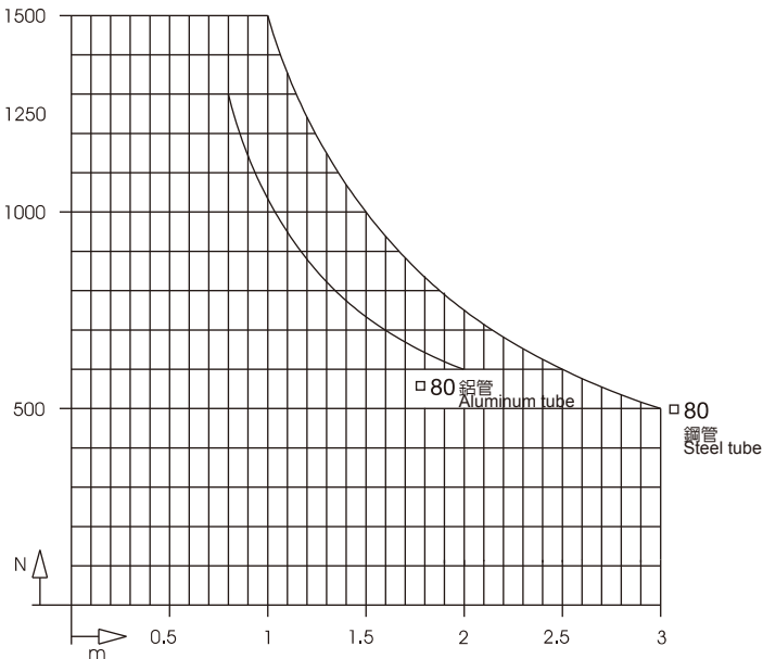
80系列重型懸臂承受力圖 Load - bearing chart of 80 series heavy support arm
