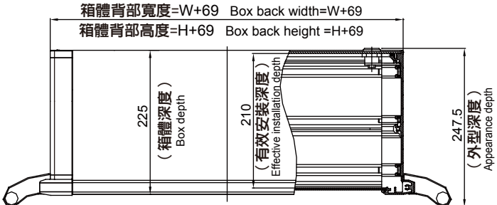
DST210 箱體尺寸(兩側把手) DST210 box size (handles on both sides)
