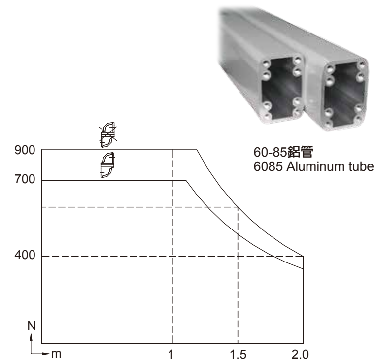
6085鋁管規格表(配6085懸臂)： Size table of 6085 aluminum tubes ( for 6085 support arms)
