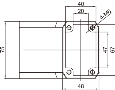
雙箱體連接管內徑尺寸： Bore size of the hard joint
