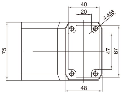
雙箱體連接管內徑尺寸圖 Bore size of the hard joint
