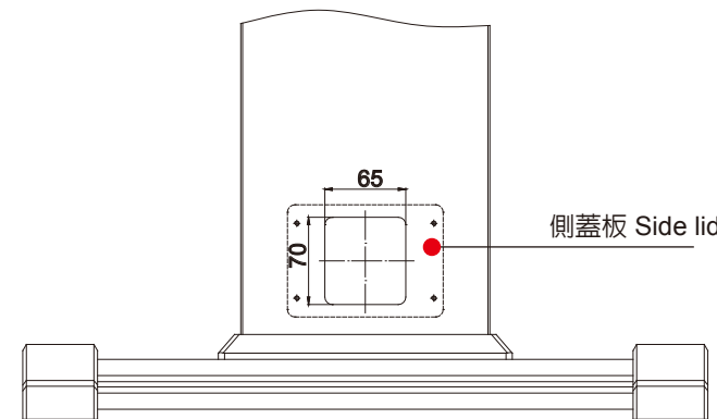
立柱下方背部 A向出線口 The outlet under the rear pillar (Direction A)
