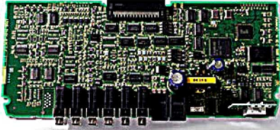
FANUC SPINDLE SIDE PLATE
