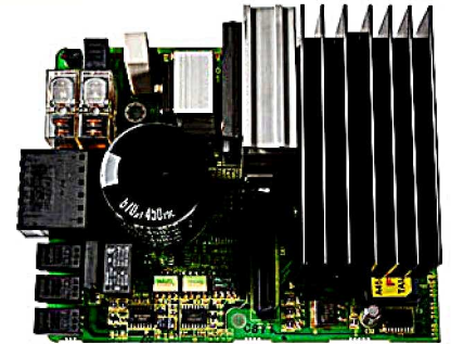
FANUC BACKPLANE
