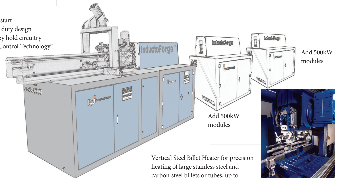
Heavy-duty twin chain tractor in-feed drive
