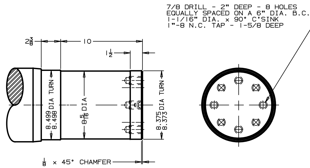
DETAIL OF RAM NOSE SCALE: 3"=1'-0"
