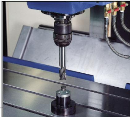
Automatic tool length measuring device
