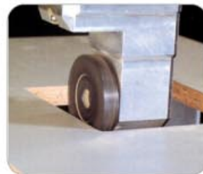
▲ Benz aggregate head BENZ複合刀軸
