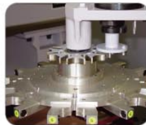
▲ Drum type 12 tools aluminum alloy tool magazine 12支鋁合金刀庫
