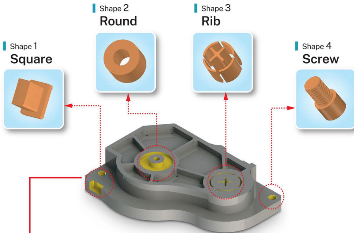
▲ Single mold, multiple machining jobs
