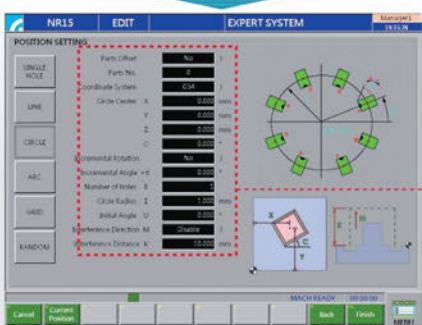
▲ Interference avoidance function
