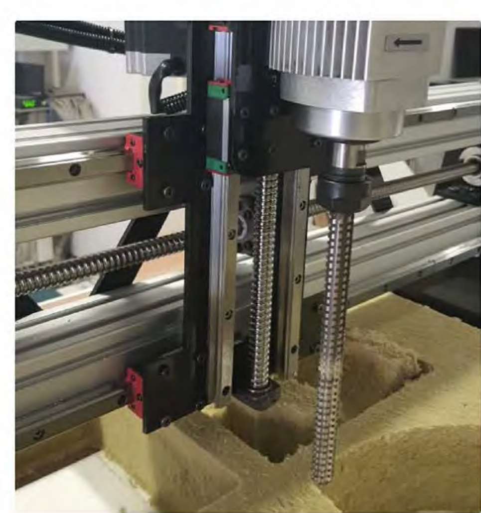
3D Rockwool Milling Machine / 3D-Steinwolle fräsmaschine
