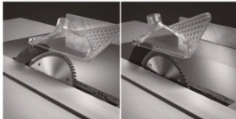
45°-90°角度切割 cut angles from 45° to 90°
