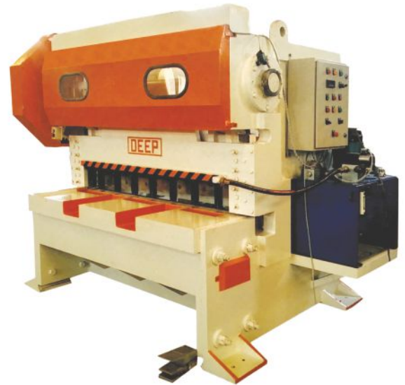
Hybrid Shearing Machine Upto 25 mm Thickness & 4000 mm Width
