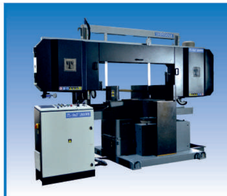
Horizontal Both Side Mitre/Swivel Beam Cutting Bandsaw Machine Model ITL-18x27 LMGSWM
