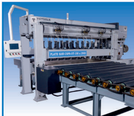
Plate Cutting Circular Saw Machine Model ITL-CSPS-OT-100x2500
