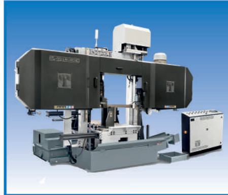
Fully Automatic Horizontal Double Column Bandsaw Machine Model ITL-660 TCBA-NC
